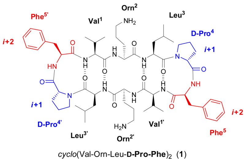
Figure 1. Structure of gramicidin S (top) and the analog generated (1) by sequence inversion at the \beta -turn (bottom). In both cases the peptide adopts \beta -sheet structure.
