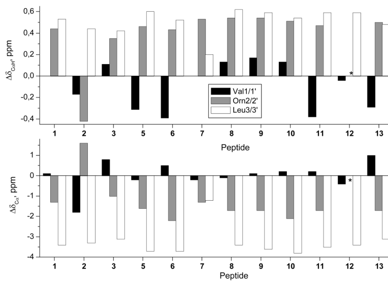
Figure 4. \Delta\delta_{C\alpha H} and \Delta\delta_{C\alpha} profiles ( \Delta\delta = \delta^{\text{observed}} - \delta^{\text{random coil}} , ppm) for GS analogs in aqueous solution at pH 3.0 and 5 °C. Lys \delta^{\text{random coil}} values 43 were used to calculate the \Delta\delta values for the Orn residues. The \delta_{C\alpha H} and \delta_{C\alpha} values for the Orn residues in 12 could not be assigned.
