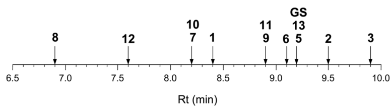
Figure 5. Retention times (Rt) of GS analogs on RP-HPLC. Elution conditions: see experimental section. The retention time of GS under the same conditions is also shown for comparison.
