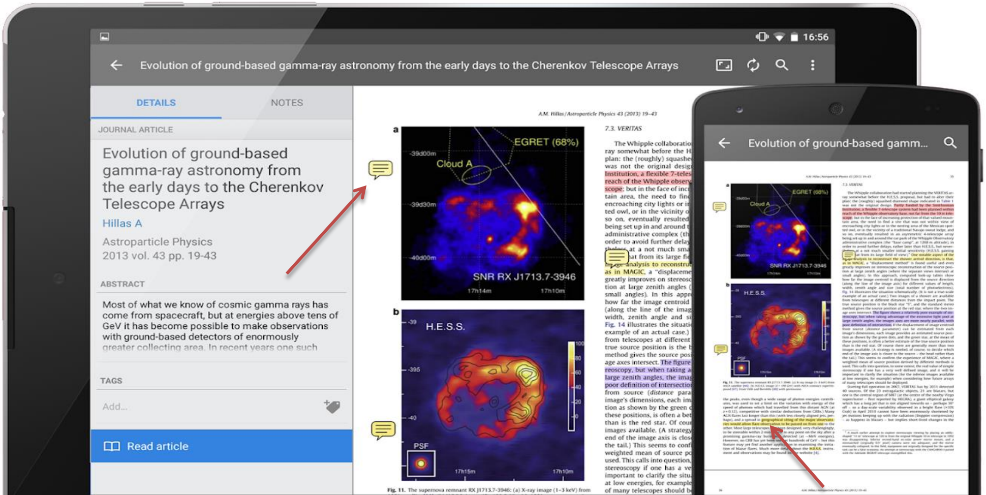
Fig. 11. The supernova remnant RX J1713.7-3946: (a) X-ray image (1–3 keV) from
