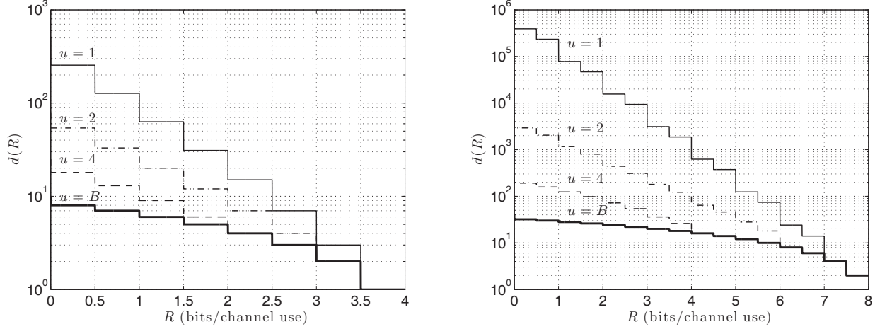
Fig. 1. The effect of u on outage diversity for an M = 4 , B = 8 system: (left) SISO channel; (right) 2 \times 2 MIMO channel.
