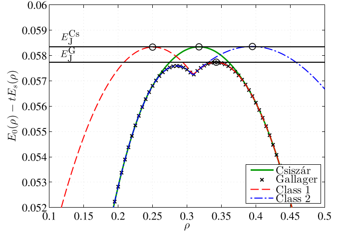
Fig. 1. Error exponent bounds. Csiszár's and Gallager's curves correspond to \bar{E}_0(\rho, W) - tE_s(\rho, P) and E_0(\rho, W) - tE_s(\rho, P) , respectively. Class i curves correspond to E_0(\rho, W) - \lim_{n \rightarrow \infty} \frac{1}{n} E_s^{(i)}(\rho, P^k) , for i = 1, 2 .
