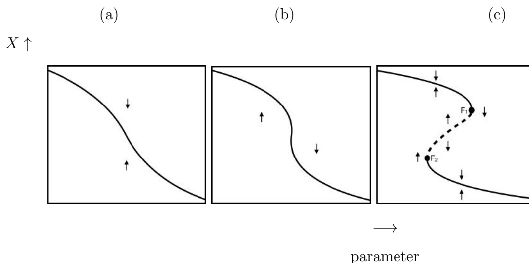
Figure 1: Panel (a): When nonlinearities are mild, a change in parameters only leads to a gradual change in the stable steady state of the system; Panel (b): When nonlinearities become stronger, a small change in parameters may lead to a larger change in the stable steady state of the system, but the change is still continuous and reversible; Panel (c): With very strong nonlinearities catastrophic changes from a "good" steady state to a "bad" or "crisis" steady state of the system may occur after small changes of a parameter. At the point F_1 a catastrophic change occurs and the system jumps from the "good" stable steady state to the "bad" steady state. After such a catastrophic change, the system can not easily be recovered as pushing back the system to the "good" steady state requires that the parameter be decreased until the point F_2 , where the "bad" steady state disappears.
